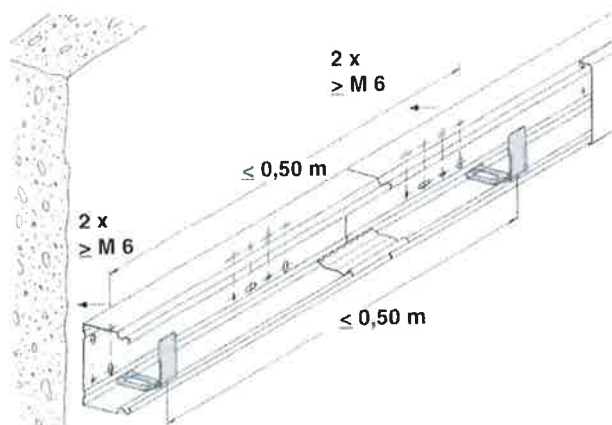
Wandmontage
