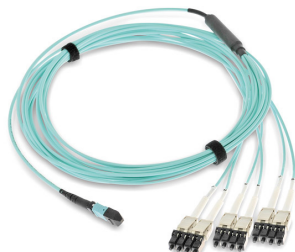
Cable fanout FO-DCS, MTP-on-LCDU, 12 fibras
