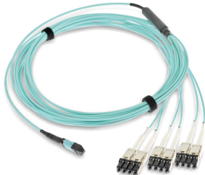
FO-DCS fanout cable, MTP-on-LCDU, 12 fibres
